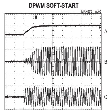
DPWM SOFT-START MAX8751 toc06 A: COMP, 1V/div B: IFB, 1V/div C: VFB, 1V/div
