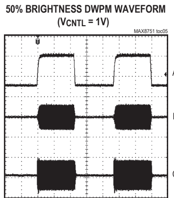
50% BRIGHTNESS DPWM WAVEFORM (VcNTL = 1V) MAX8751 toc05 A: COMP, 500mV/div B: IFB, 2V/div C: VFB, 1V/div
