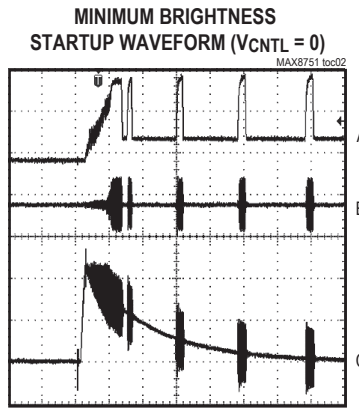
MINIMUM BRIGHTNESS STARTUP WAVEFORM (VcNTL = 0) MAX8751 toc02 A: COMP, 500mV/div B: IFB, 2V/div C: VFB, 1V/div
