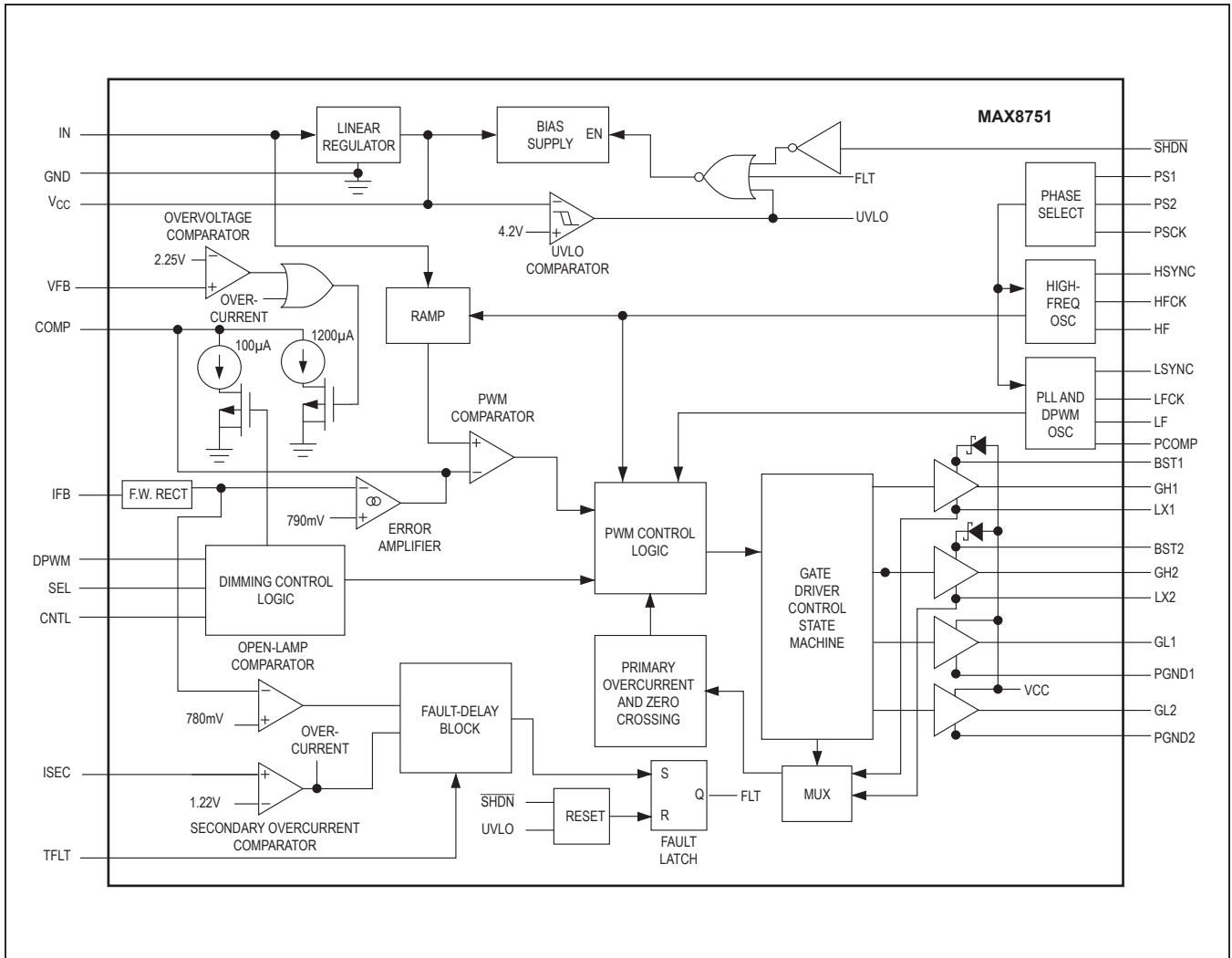
Figure 2. Functional Diagram
