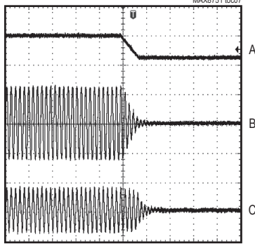
DPWM SOFT-START
