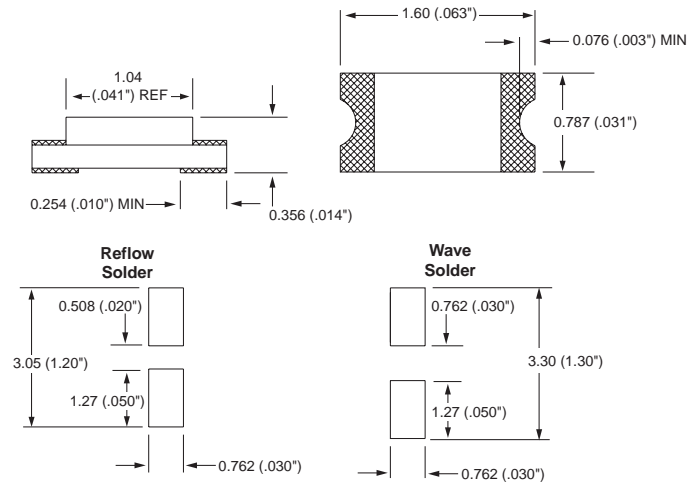
Reference Dimensions:
