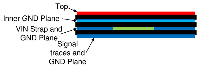
Figure 10-2. Example Layout for Fixed Output
