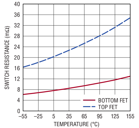
Switch Resistance
