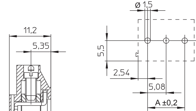
PCB LAYOUT - COMPONENT VIEW
