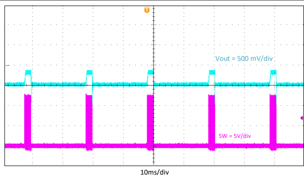
Figure 9-7. Hiccup, I_{out} = 5 A
