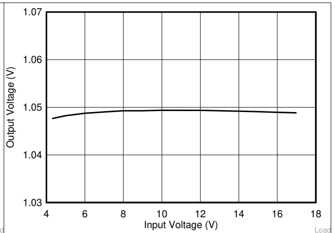
Figure 9-3. Load Regulation with Different Input Voltage
