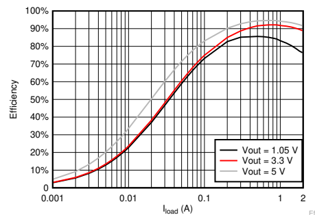
TPS562207S Efficiency
