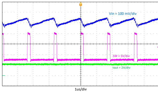
Figure 9-4. Input Voltage Ripple
