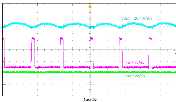
Figure 9-6. Output Voltage Ripple, I_{out} = 2 A
