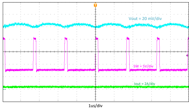
Figure 9-5. Output Voltage Ripple, I_{out} = 0.2 A
