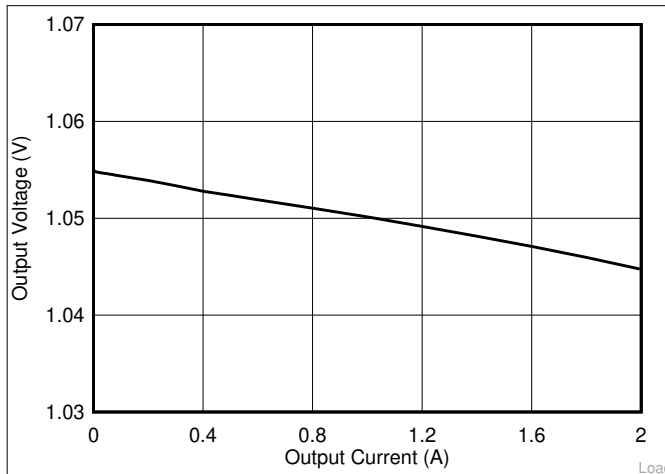
Figure 9-2. Load Regulation with Different Loading
