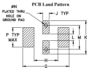
Suggested Layout, Tolerance to be within ±0.002
