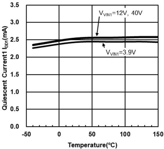
Quiescent Current1 vs Temperature R_L=No\ Load, V_{FB1}=0.9V
