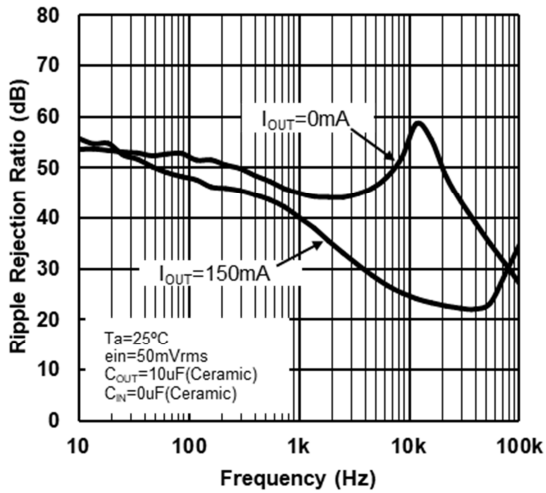
Ch.3,4 RippleRejection vs Frequency V_{OUT}=2.5\text{V}, V_{LDVIN}=3.3\text{V}
