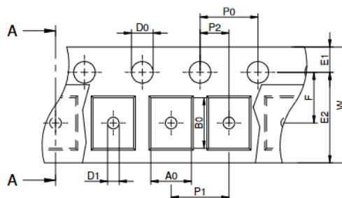
Packaging Specification - Tape: [mm]
