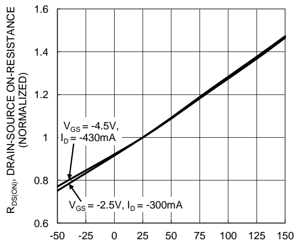
T_J , JUNCTION TEMPERATURE ( ^\circ C ) Figure 6. On-Resistance Variation with Temperature
