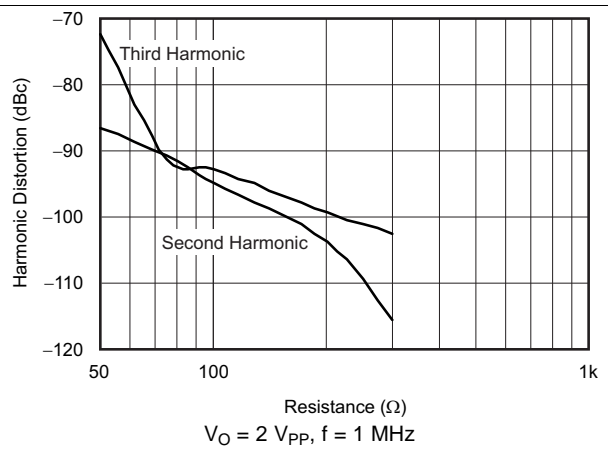
Figure 10. Harmonic Distortion vs Load Resistance
