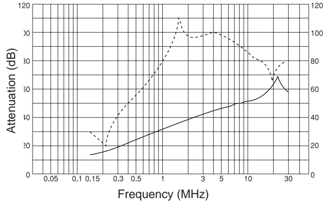
MAF-1220
