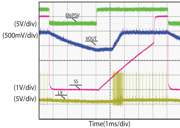
Start-up (Pre-Bias) - EN/PSV (V DD = 5 V, V IN = 12 V, V OUT = 1.5 V, I OUT = 0 A, SiC401B)
