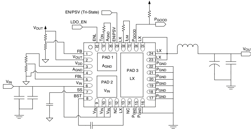
Typical Application Circuit for SiC401A/B (PowerPAK MLP32-55G)
