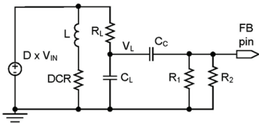
Fig. 15 - FB Voltage by CL Voltage
