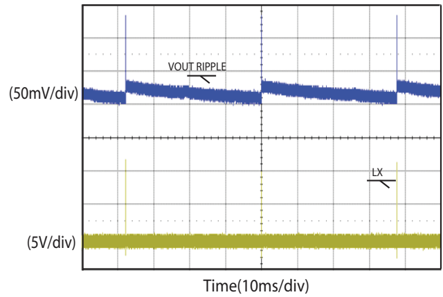
Power-Save Mode (V DD = 5 V, V IN = 12 V, V OUT = 1.5 V, I OUT = 0 A, SiC401B)
