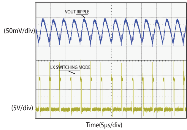
Forced Continuous Mode (V DD = 5 V, V IN = 12 V, V OUT = 1.5 V, I OUT = 15 A, SiC401B)
