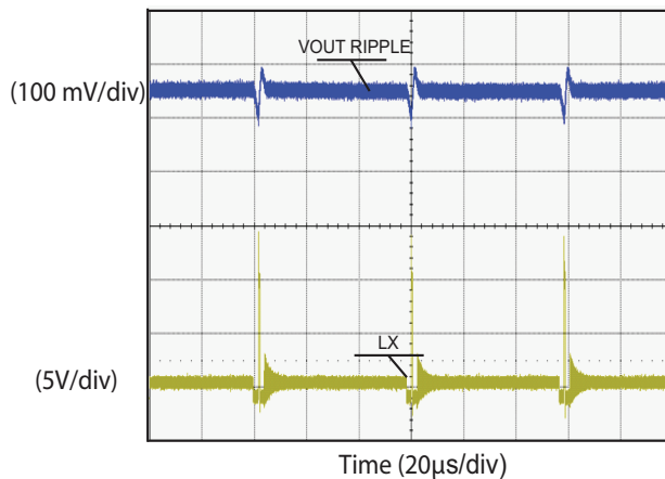
Power-Save Mode (V DD = 5 V, V IN = 12 V, V OUT = 1.5 V, I OUT = 0 A, SiC401A)
