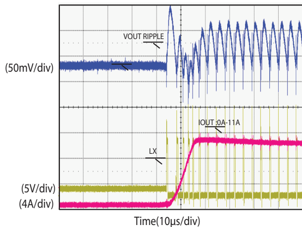
Transient Response - P-Save Load Rising (V DD = 5 V, V IN = 12 V, V OUT = 1.5 V, I OUT = 0 A to 11 A, SiC401B, dl/dt = 1 A/µs)
