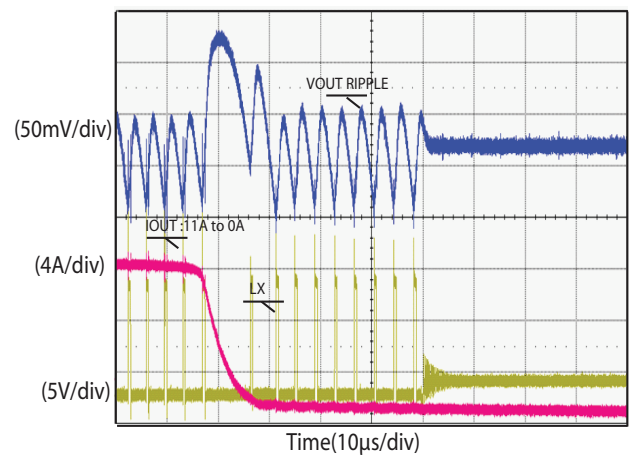
Transient Response - P-Save Load Falling (V DD = 5 V, V IN = 12 V, V OUT = 1.5 V, I OUT = 11 A to 0 A, SiC401B, dl/dt = 1 A/µs)
