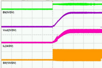
Time -10ms/div
