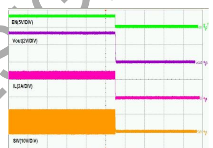
Time -5ms/div
