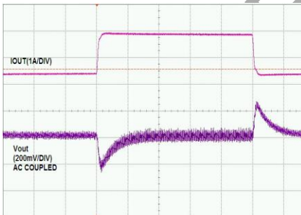
Time -100µs/div
