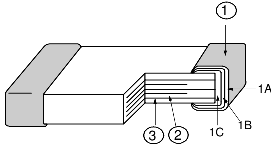
Fig.1 (Nickel Barrier termination)
