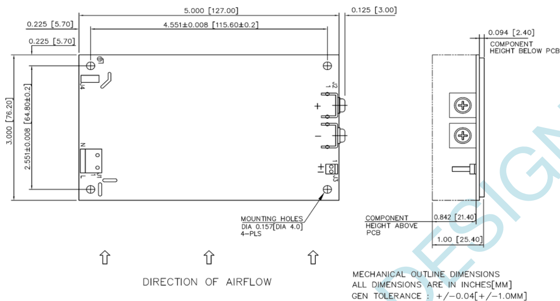
Figure 1. Mechanical Drawing - Screw Terminal (Option 1)
