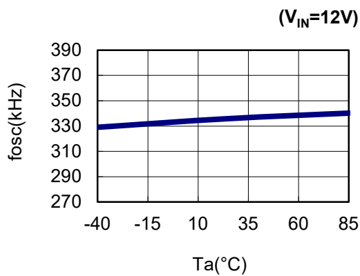
5)Oscillator Frequency(ver.C,D)
